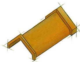
Steep Pitch Vee Ridge (81°) For roofs over 45° in pitch Dimensions: 430L x 265W x 185D Cover length: 400
